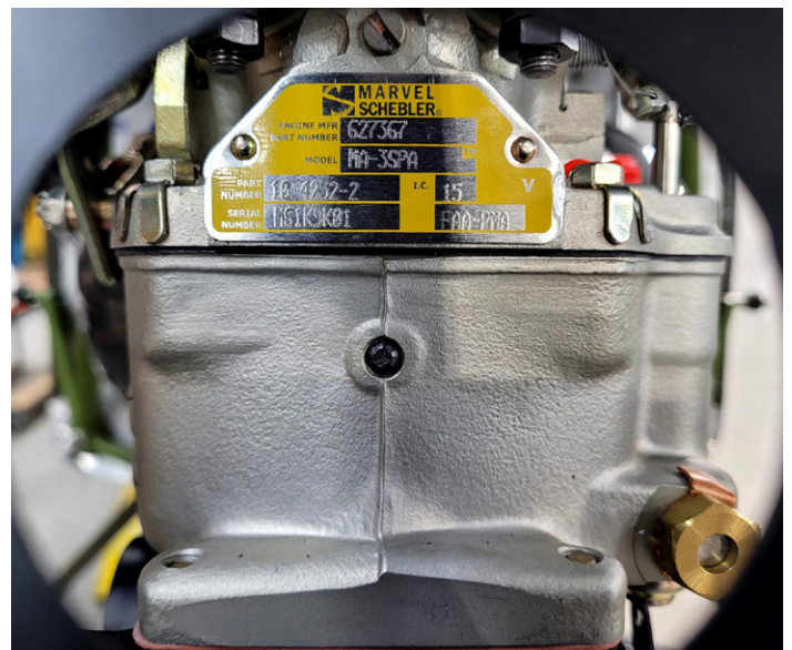
The carburetor is a Marvel Schebler MA-3SPA
