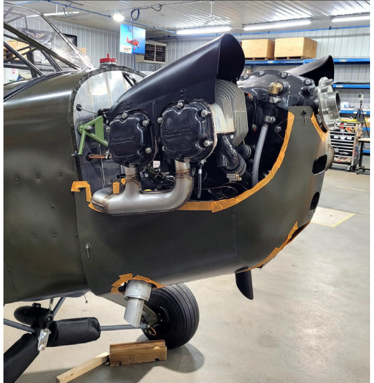
Exhaust and lower cowl are installed.
